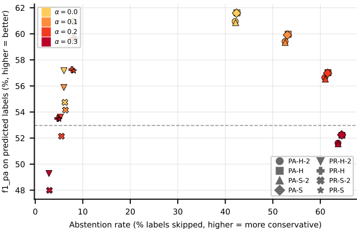
RF on Water-quality (f1_pa)
