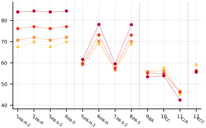
micro_recall
