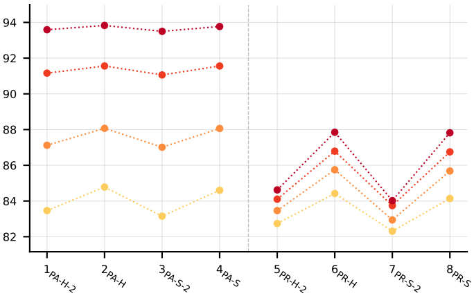
micro_recall_pa
