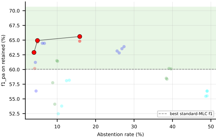
LGBM on CHD_49 (f1_pa) -- Pareto frontier + win-region
