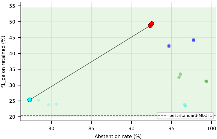
LGBM on PlantPseAAC (f1_pa) -- Pareto frontier + win-region
