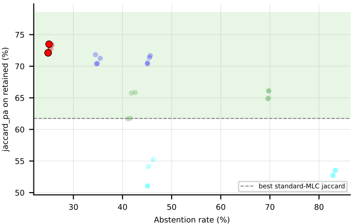
LGBM on GpositivePseAAC (jaccard_pa) -- Pareto frontier + win-region
