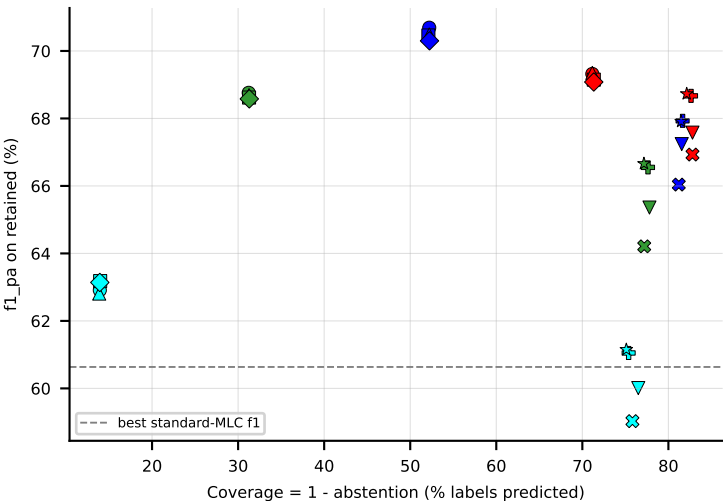
RF on emotions (f1_pa) -- robustness: upper-right = robust
