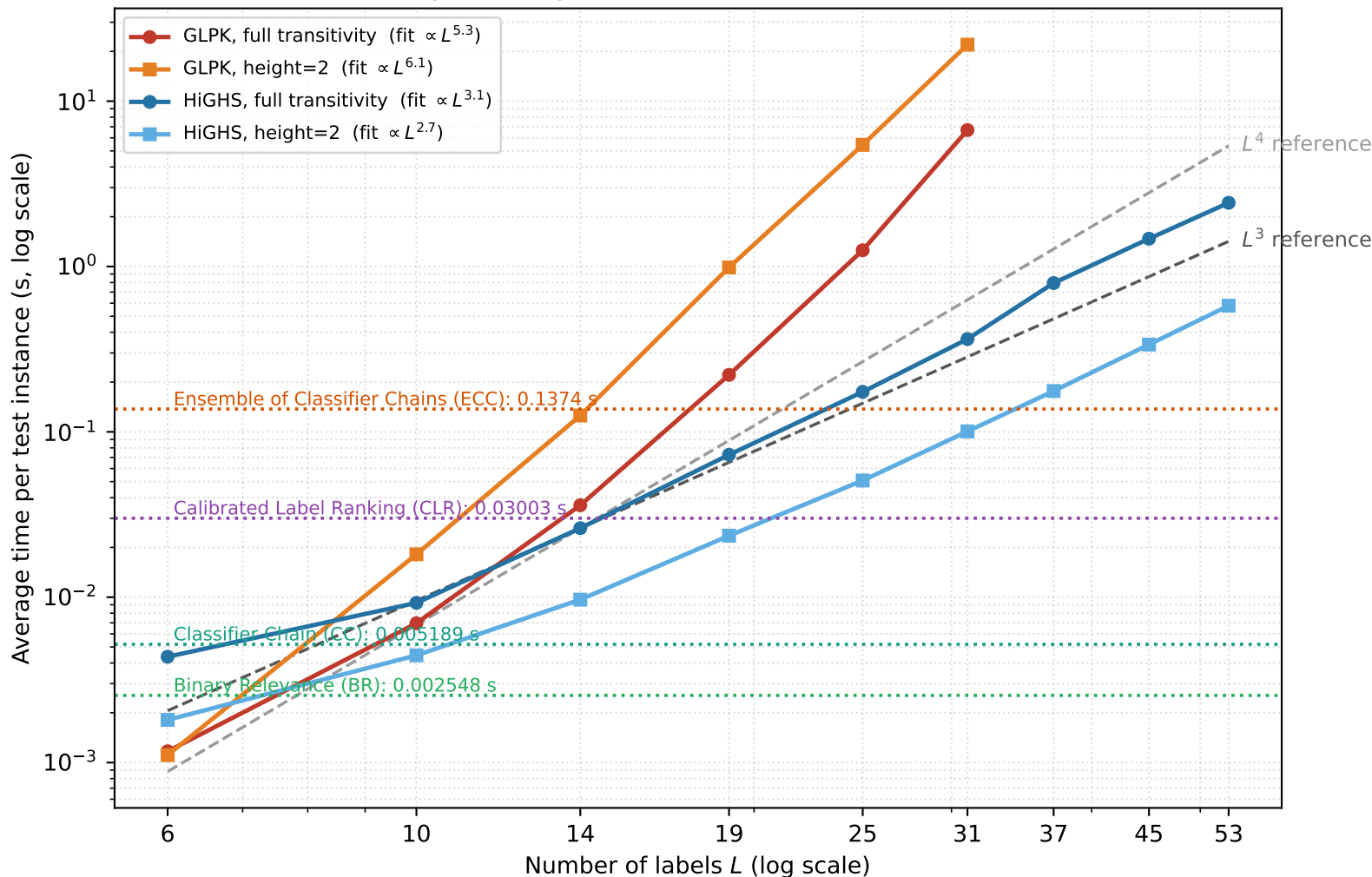
Per-instance ILP runtime scaling -- Hamming accuracy (real enron RF pairwise probabilities, mean over 300 test instances)
