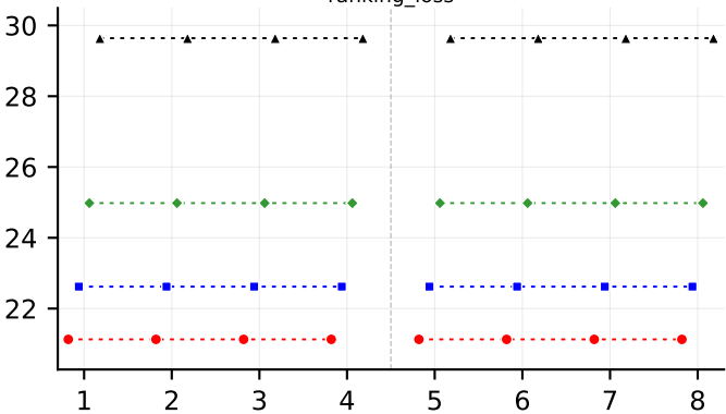
ranking_loss
