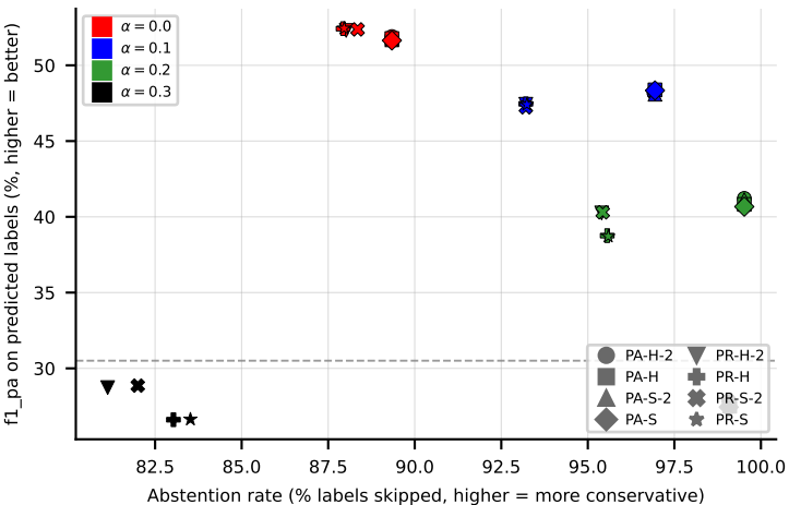
LGBM on HumanPseAAC (f1_pa)
