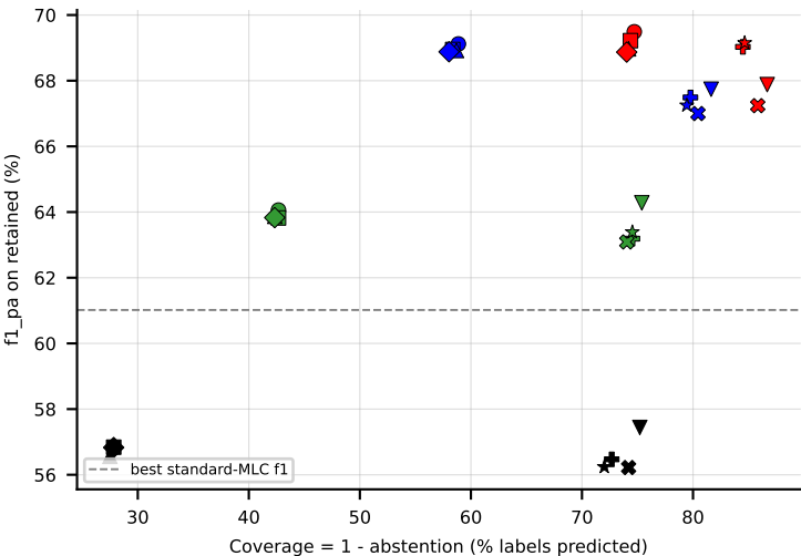
LGBM on emotions (f1_pa) -- robustness: upper-right = robust
