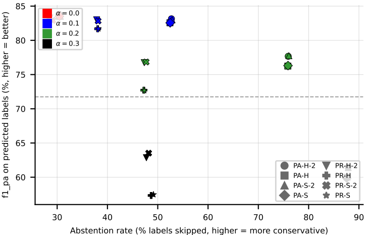
LGBM on scene (f1_pa)
