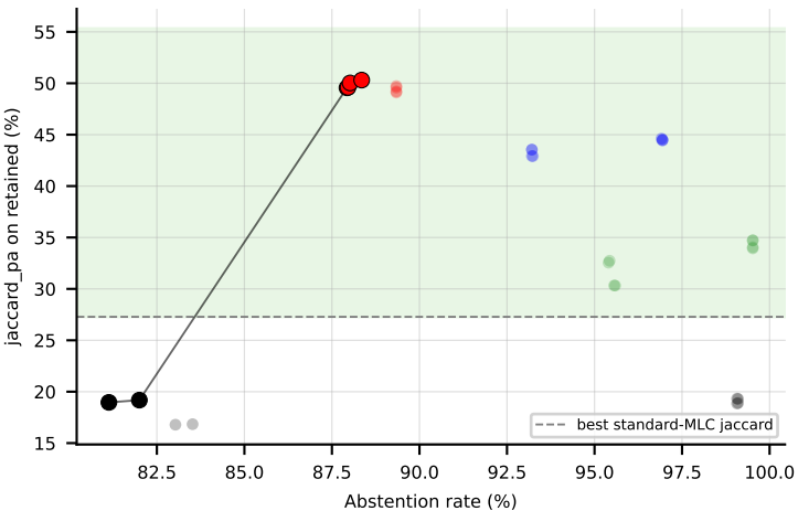
LGBM on HumanPseAAC (jaccard_pa) -- Pareto frontier + win-region
