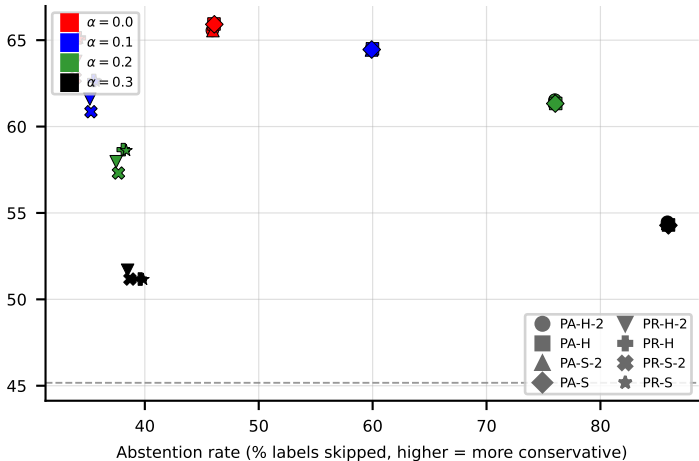
RF aggregate (f1_pa)
