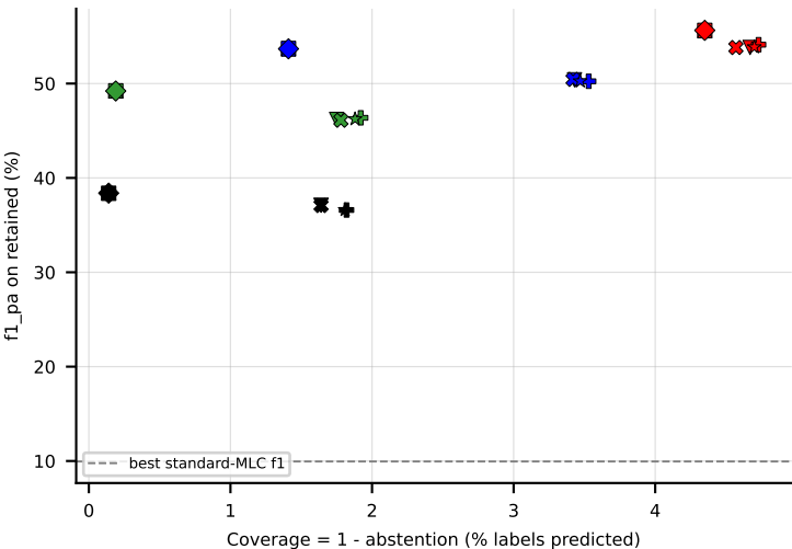
RF on HumanPseAAC (f1_pa) -- robustness: upper-right = robust
