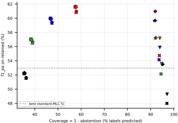
RF on Water-quality (f1_pa) -- robustness: upper-right = robust
