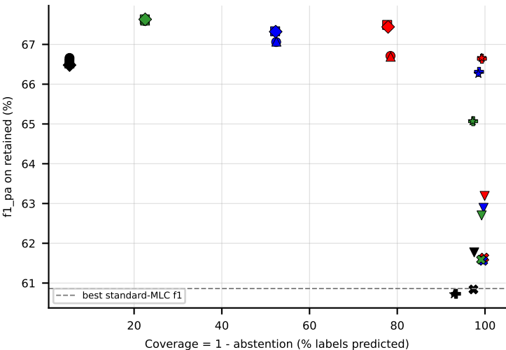
RF on Yeast (f1_pa) -- robustness: upper-right = robust
