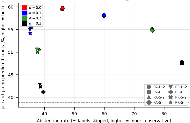
RF aggregate (jaccard_pa)
