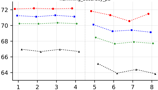
hamming_accuracy_pa
