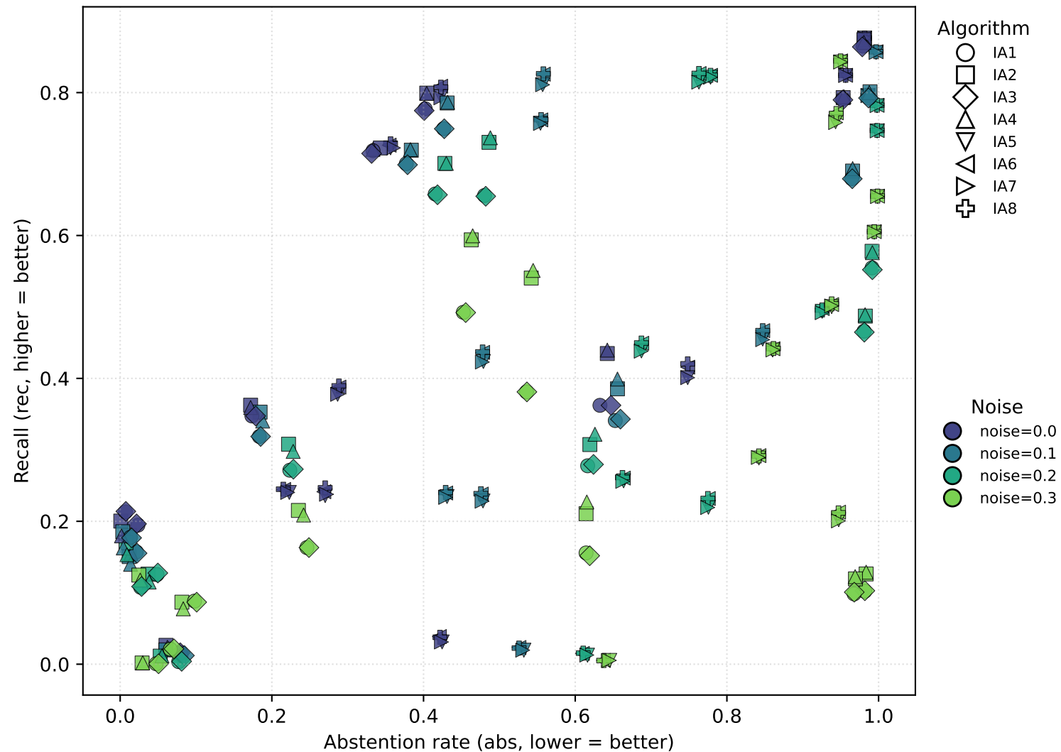
Abstention vs recall
