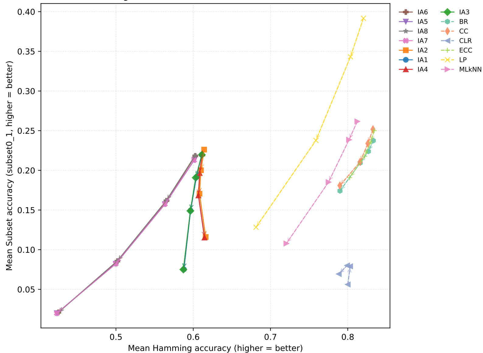
Hamming vs Subset trade-off (arrows: noise 0.0 → 0.3)
