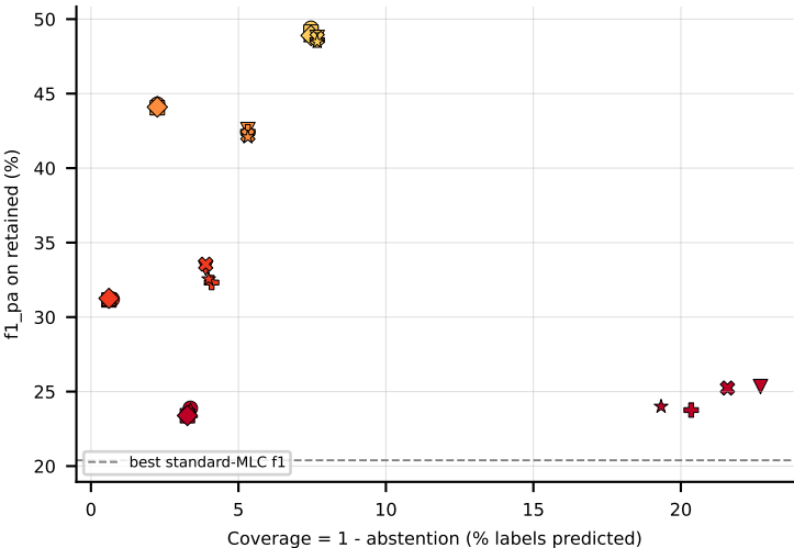
LGBM on PlantPseAAC (f1_pa) -- robustness: upper-right = robust
