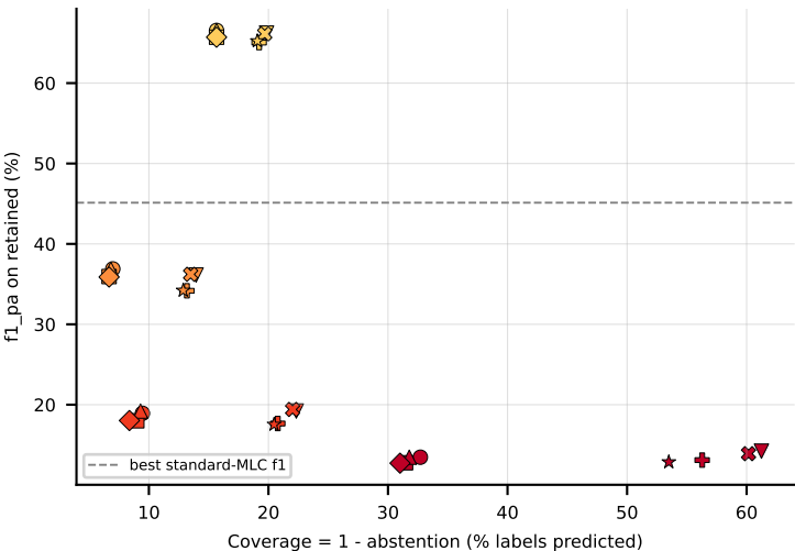
LGBM on birds (f1_pa) -- robustness: upper-right = robust
