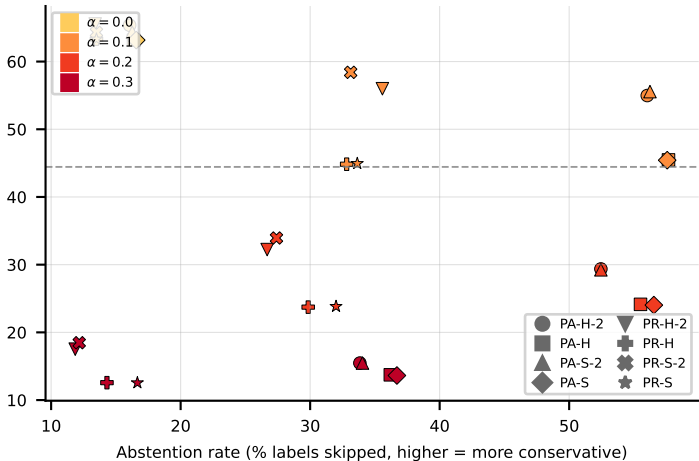
LGBM on medical (f1_pa)
