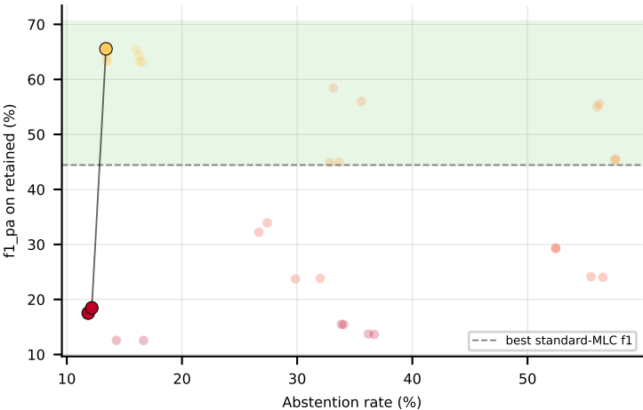
LGBM on medical (f1_pa) -- Pareto frontier + win-region
