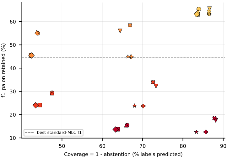
LGBM on medical (f1_pa) -- robustness: upper-right = robust
