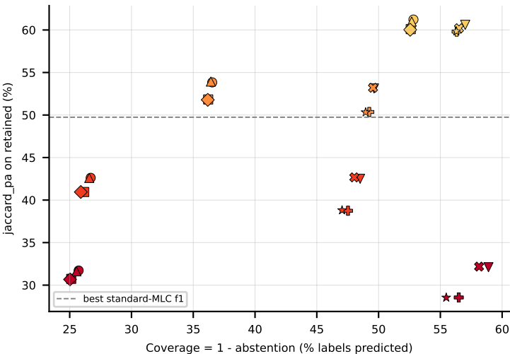
LGBM aggregate (jaccard_pa) -- robustness: upper-right = robust
