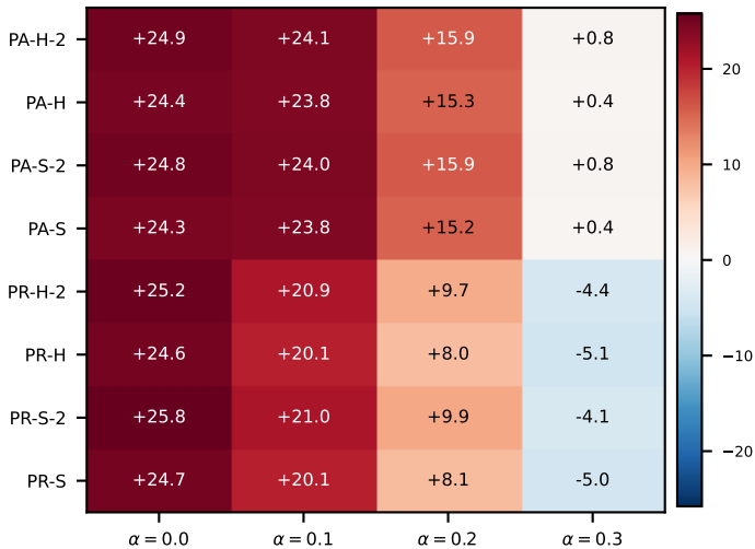
LGBM on HumanPseAAC (jaccard_pa) -- gain (jaccard_pa - f1, percentage points)
