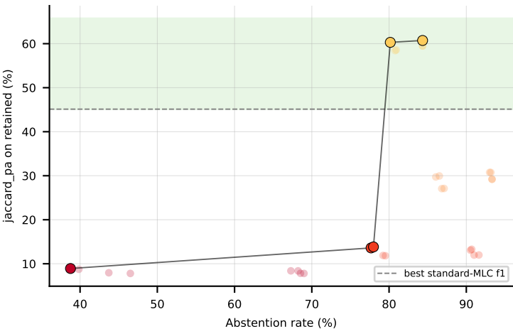
LGBM on birds (jaccard_pa) -- Pareto frontier + win-region
