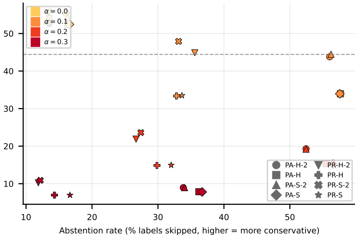
LGBM on medical (jaccard_pa)
