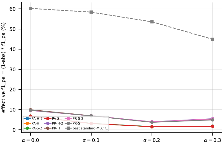
RF on birds (f1_pa) -- penalised quality (abstention costs labels)
