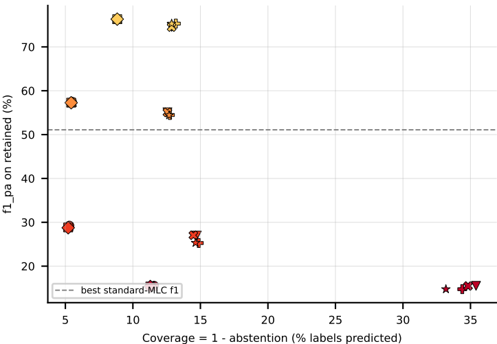
RF on birds (f1_pa) -- robustness: upper-right = robust
