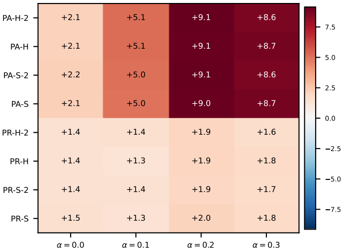
RF on emotions (f1_pa) -- gain (f1_pa - f1, percentage points)
