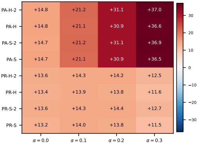
RF on scene (f1_pa) -- gain (f1_pa - f1, percentage points)
