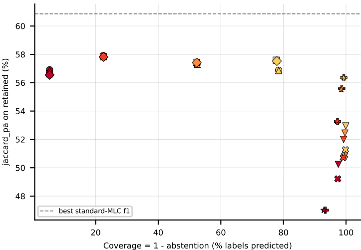
RF on Yeast (jaccard_pa) -- robustness: upper-right = robust
