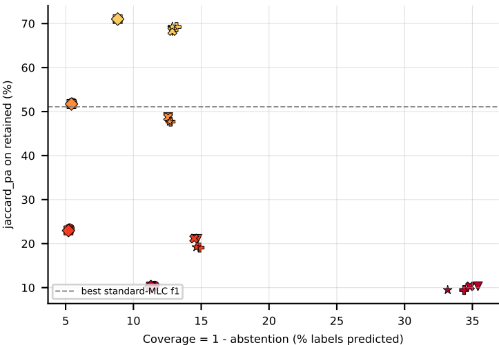
RF on birds (jaccard_pa) -- robustness: upper-right = robust
