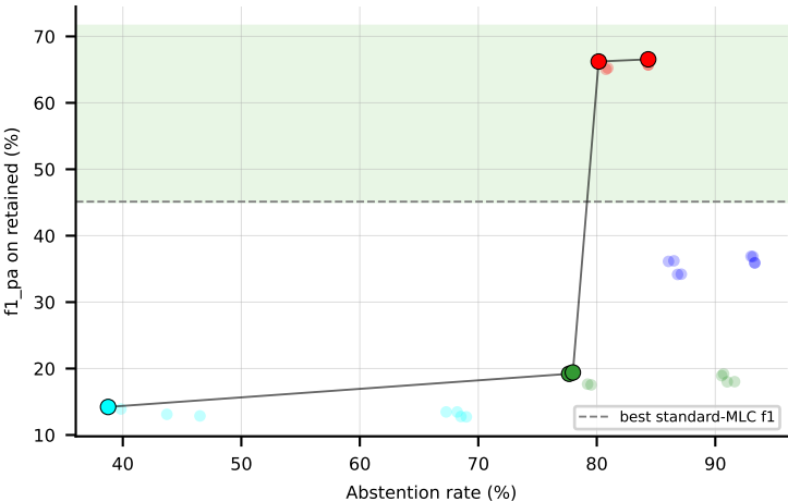
LGBM on birds (f1_pa) -- Pareto frontier + win-region
