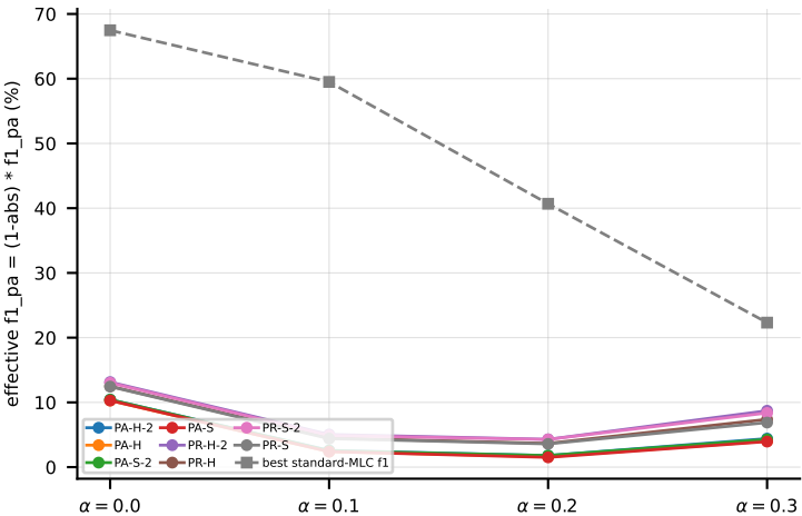
LGBM on birds (f1_pa) -- penalised quality (abstention costs labels)
