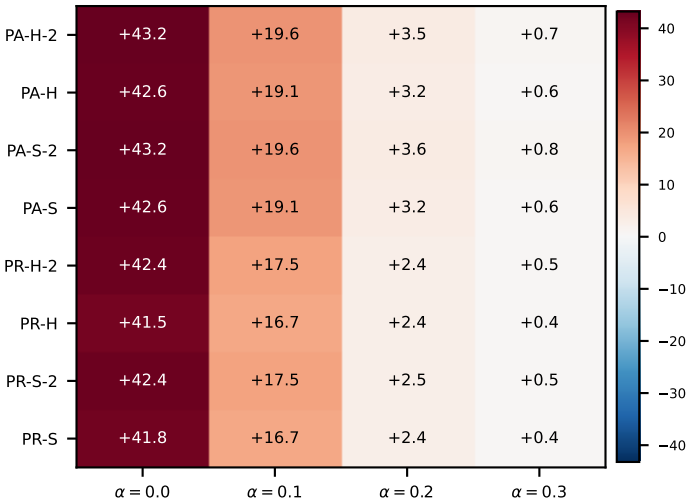
LGBM on birds (f1_pa) -- gain (f1_pa - f1, percentage points)
