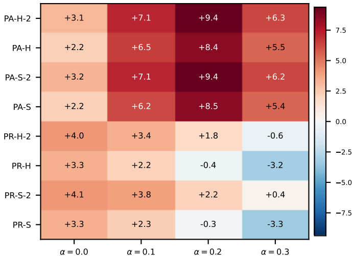
LGBM on GpositivePseAAC (jaccard_pa) -- gain (jaccard_pa - f1, percentage points)
