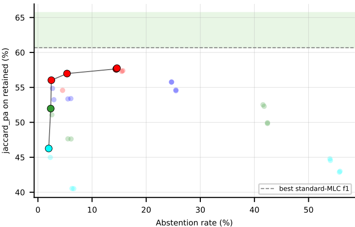
LGBM on Yeast (jaccard_pa) -- Pareto frontier + win-region
