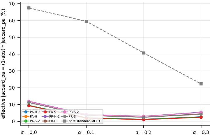
LGBM on birds (jaccard_pa) -- penalised quality (abstention costs labels)
