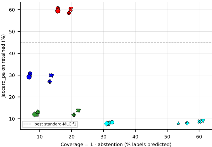
LGBM on birds (jaccard_pa) -- robustness: upper-right = robust
