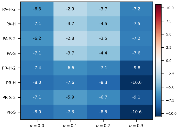
LGBM on emotions (jaccard_pa) -- gain (jaccard_pa - f1, percentage points)
