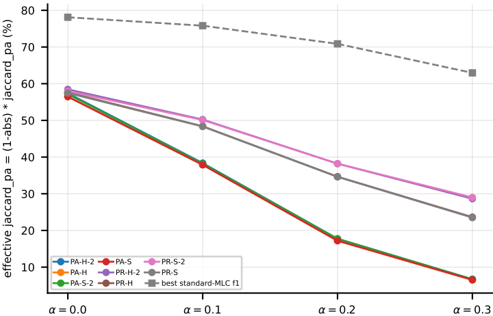
LGBM on scene (jaccard_pa) -- penalised quality (abstention costs labels)
