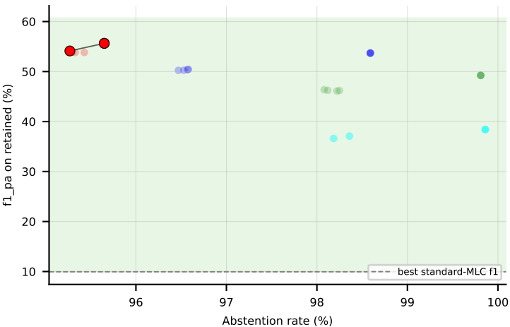
RF on HumanPseAAC (f1_pa) -- Pareto frontier + win-region
