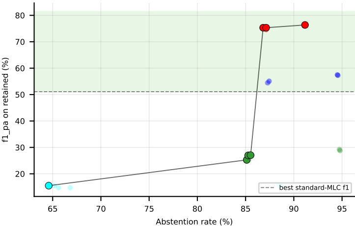
RF on birds (f1_pa) -- Pareto frontier + win-region
