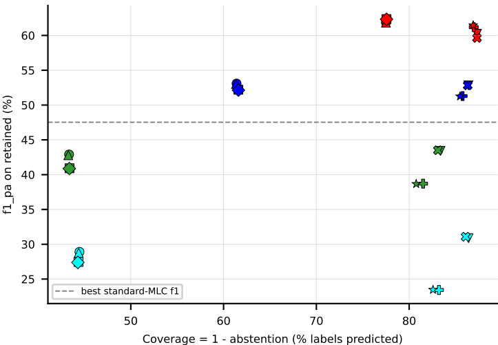
RF on enron (f1_pa) -- robustness: upper-right = robust
