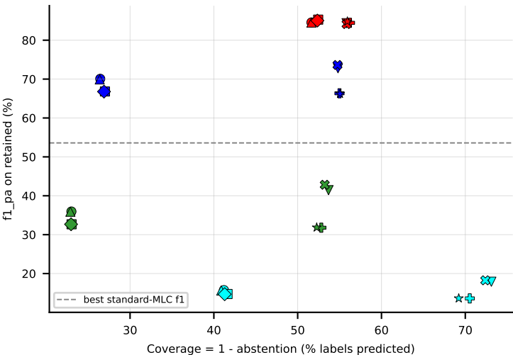
RF on medical (f1_pa) -- robustness: upper-right = robust
