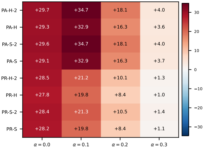
RF on medical (f1_pa) -- gain (f1_pa - f1, percentage points)
